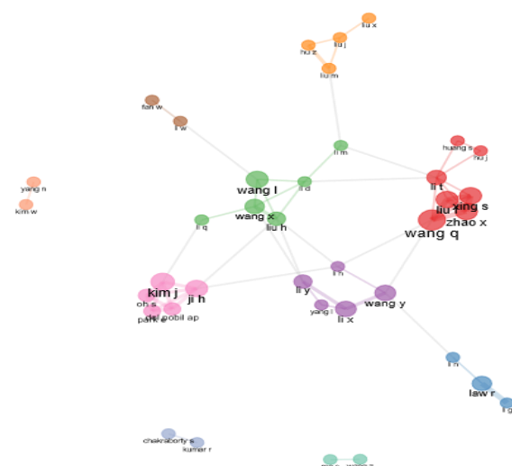
Figure 9. Co-occurrence Network
