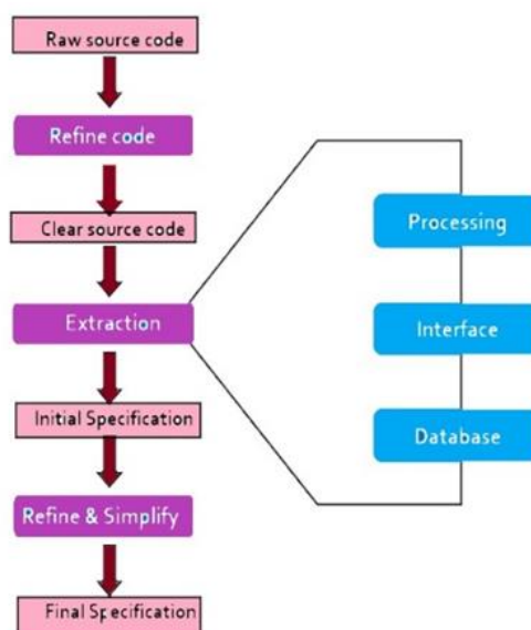
Figure 3. Process of Reverse learning [8]
