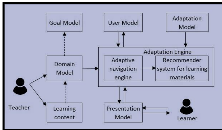
Figure 7. Architectural overview of Adaptive Machine Learning
