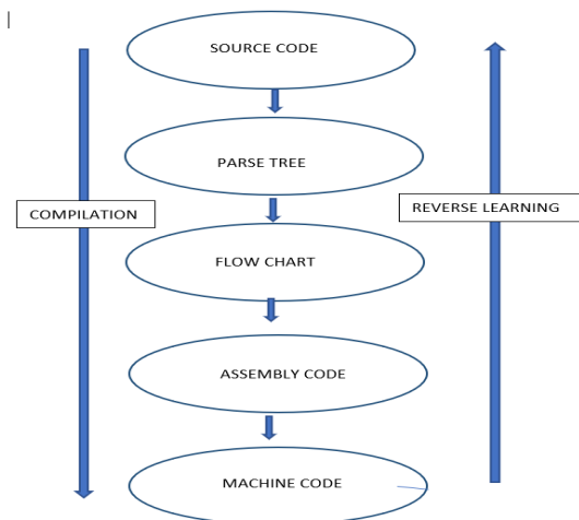
Figure 1. Architectural overview of Reverse Learning
