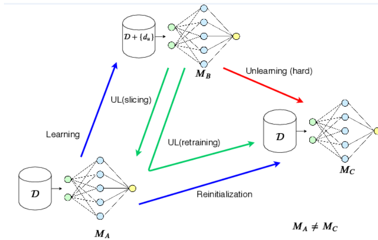
Figure 4. Machine Unlearning Technique [8]
