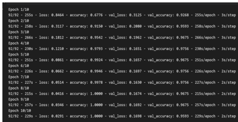
Figure 9. Model Accuracy
