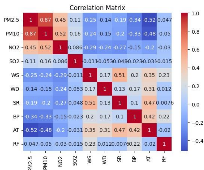
Figure 3. Correlation Matrix
