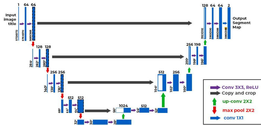
Figure 2. UNet Architecture. [21]
