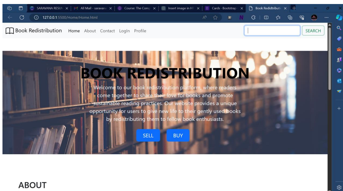
Figure 5. Home Page
