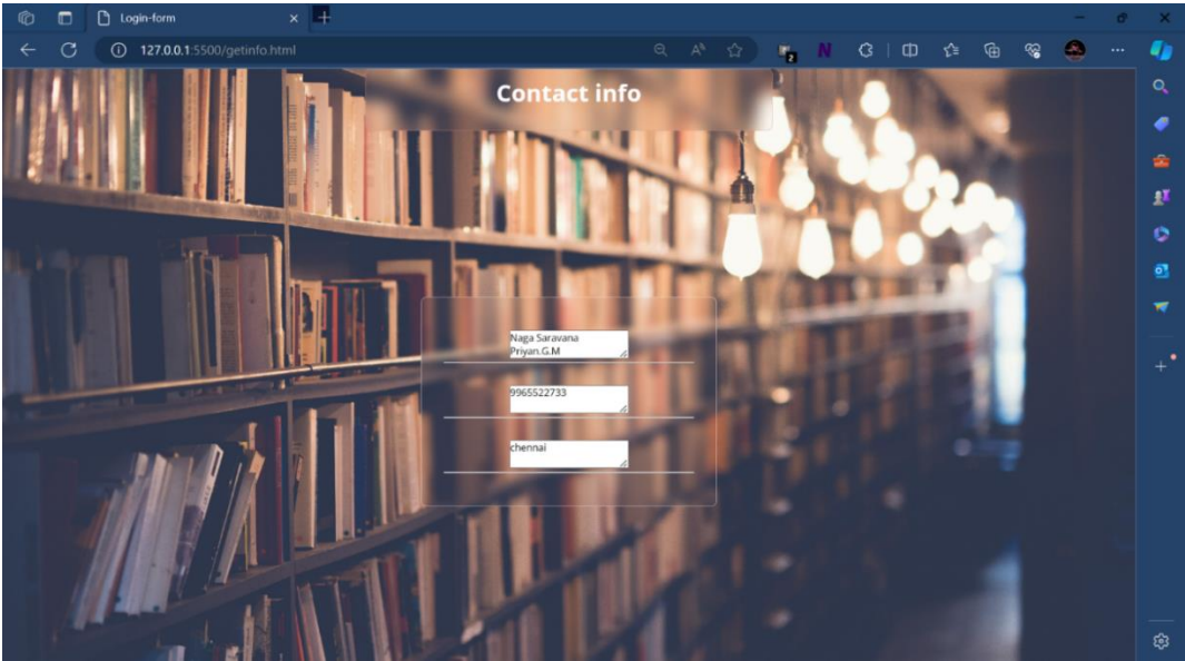
Figure 7. Result Page
