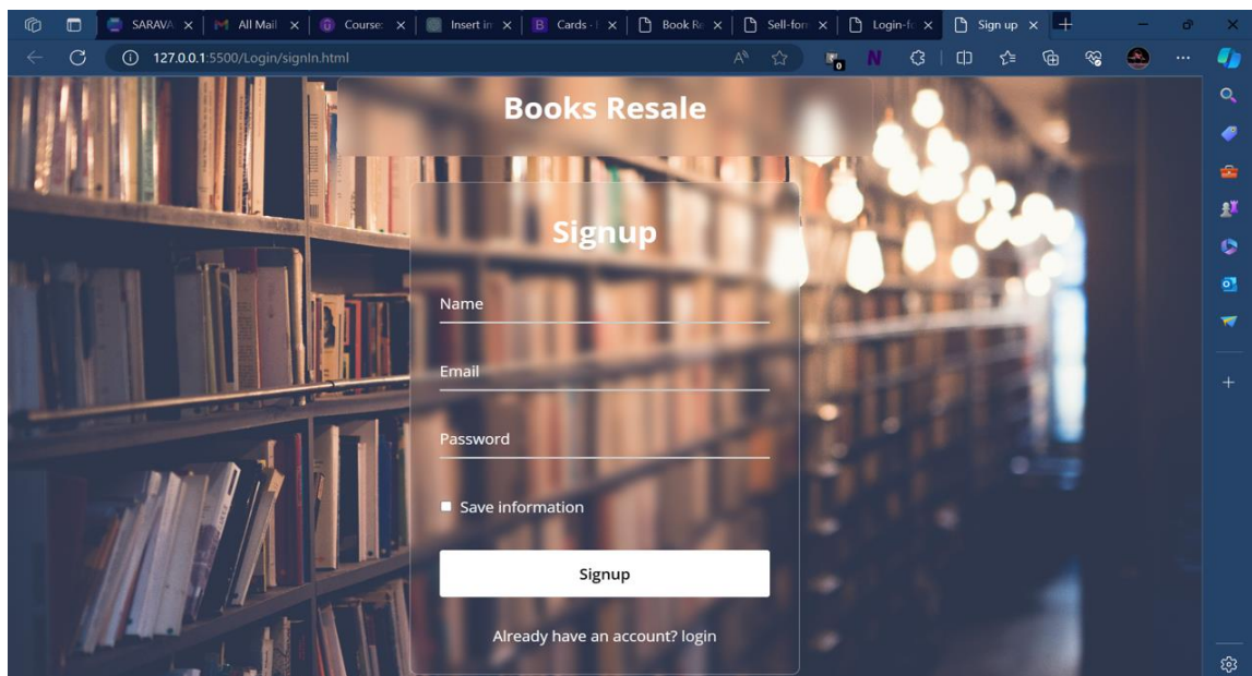
Figure 4. Signup Page
