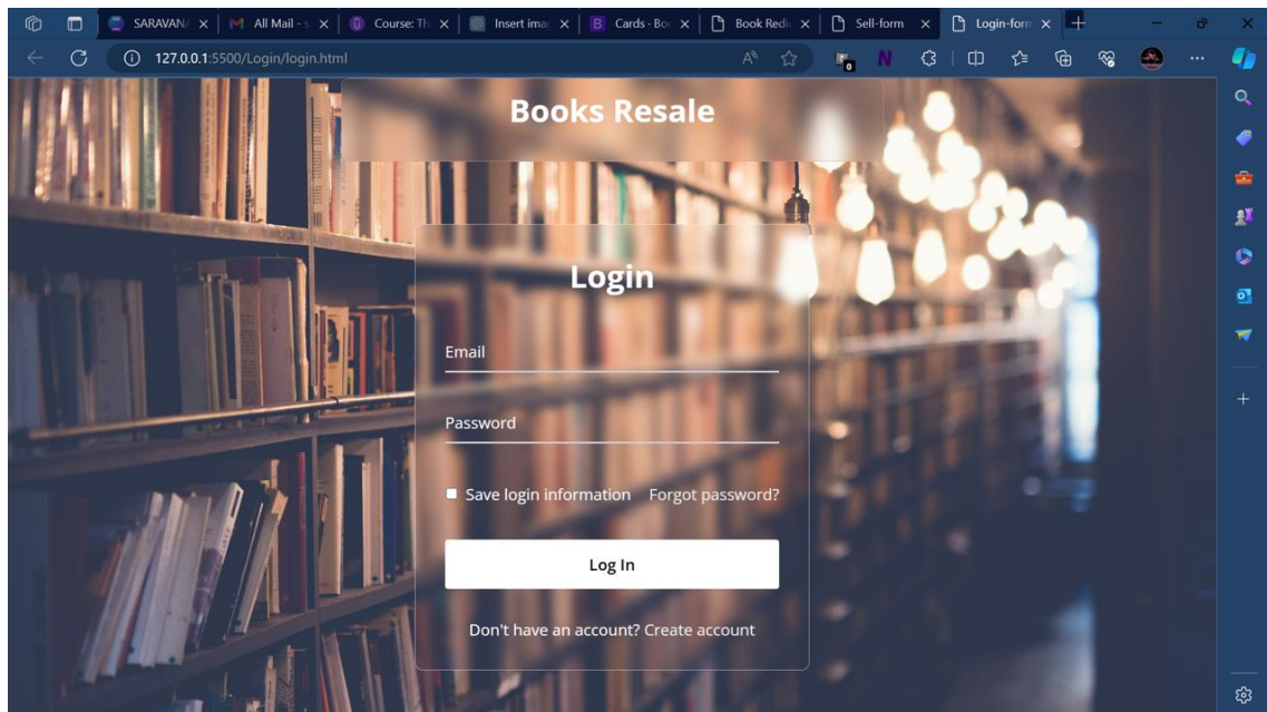
Figure 3. Login Page
