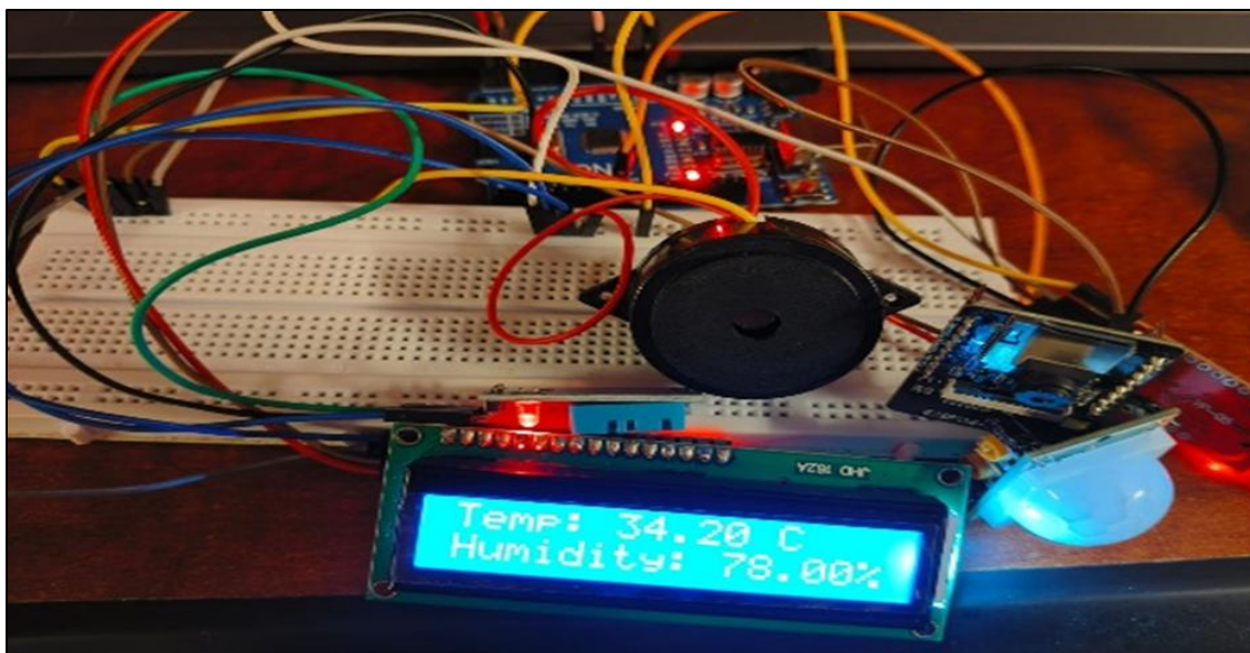
Figure 12. Hardware Module
