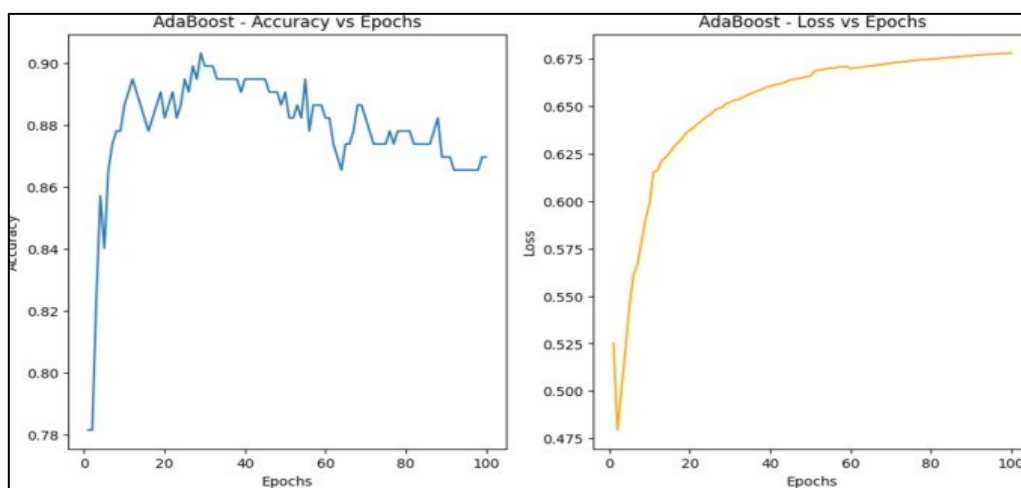
Figure 4. AdaBoost-Accuracy & Loss for Each Epochs
