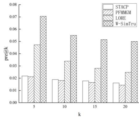
(a) NYC-precision@k
