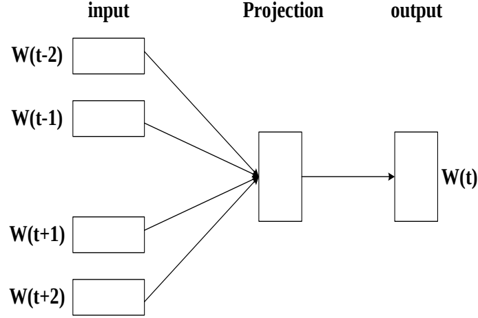
Figure 1. CBOW model
