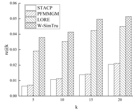
(b) Washington-recall@k
