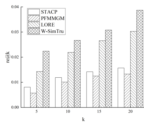
(b) NYC-recall@k
