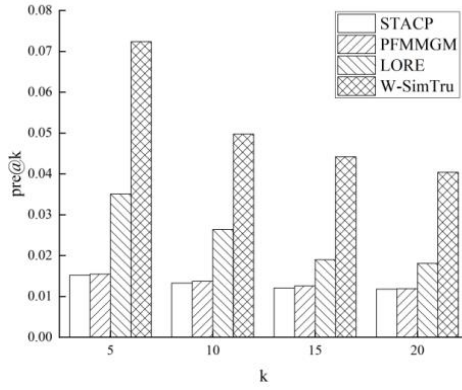
(a) Washington-precision@k
