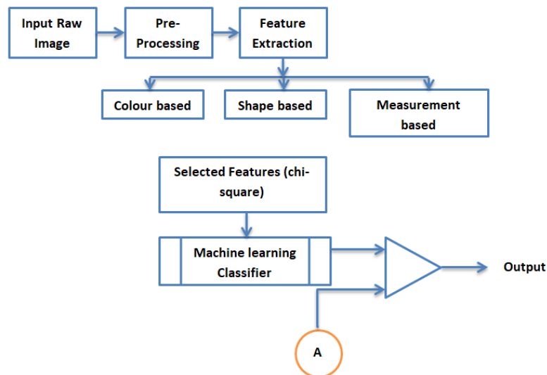
Figure 4 Proposed work of Phase 2
