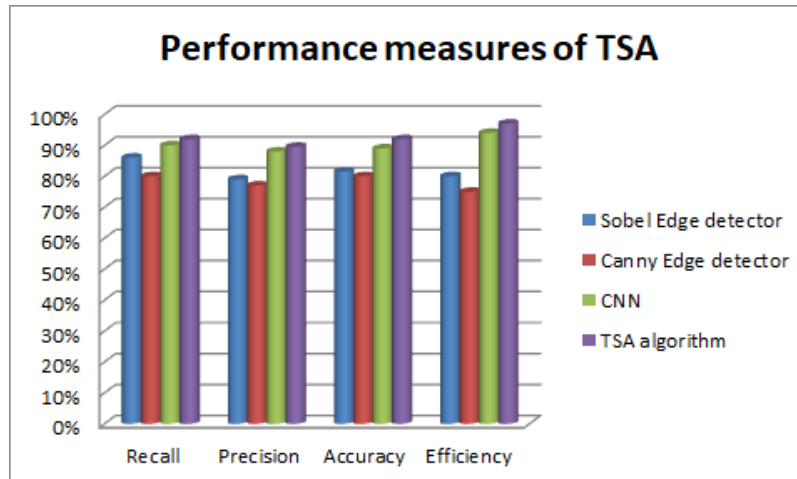
Figure 8 Overall Performance Analysis of Proposed Method
