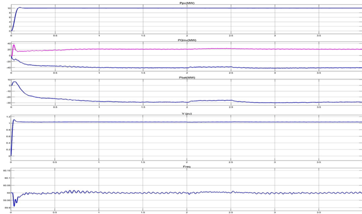
Figure 15. PV output power, active and reactive power of inverter, battery power, 14 th bus voltage waveform and frequency waveform in 2 nd scenario
