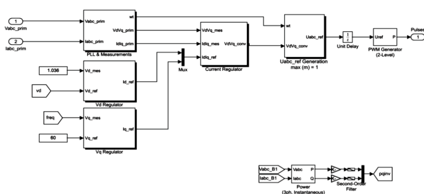
Figure 4. VSC Control scheme
