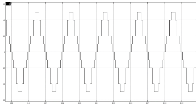
Figure 5.2 Sinusoidal Like Output Voltage (BS Unit)
