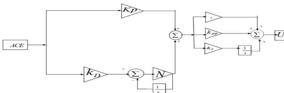
Figure 3. MPID Structure [16]
