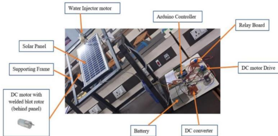
Figure 4. Hardware Prototype
