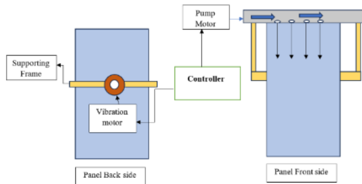
Figure 2. Model Diagram of Vibration and Water Pump Setup in Solar Panel.
