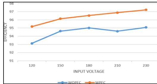
Figure 12. Comparison of Efficiency With and Without PFC
