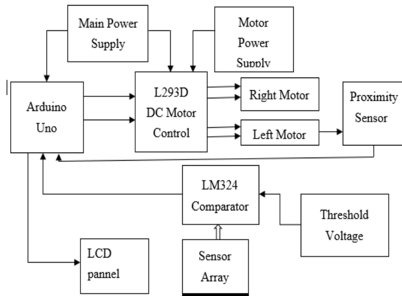
Figure 1. Block diagram of the line following robot
