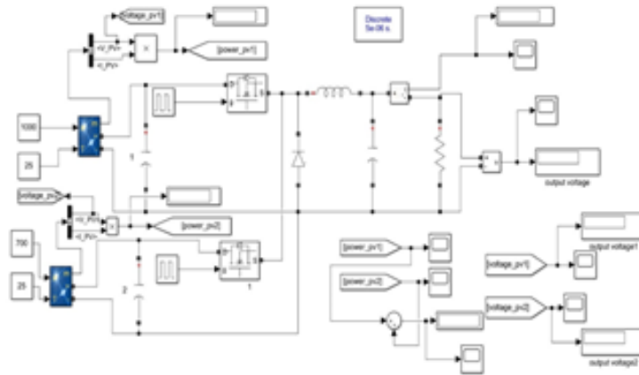
Figure 4. Simulation for P&O
