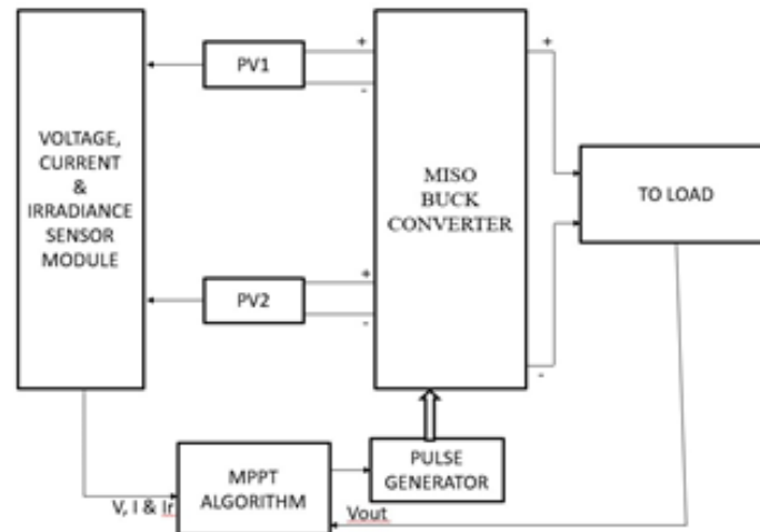
Figure 1. Block diagram for a PV system's MPPT implementation
