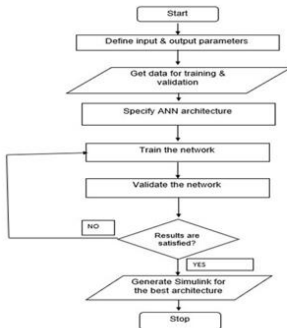
Figure 3. Flowchart of Artificial Neural Network Algorithm
