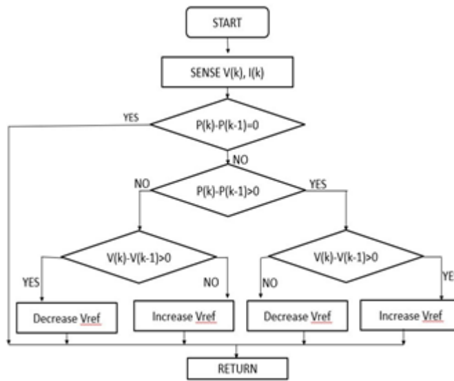
Figure 2. Flowchart of P&O
