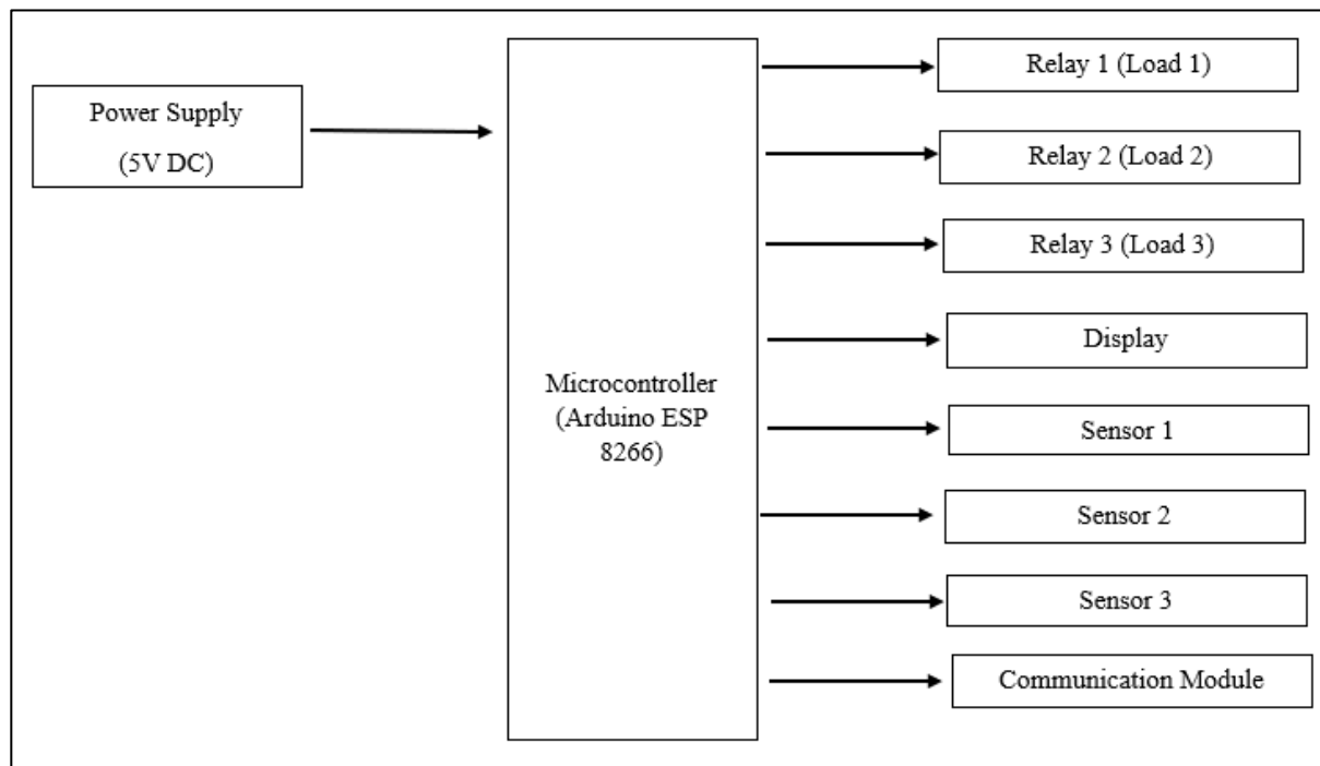
Figure 3. Hardware Connections
