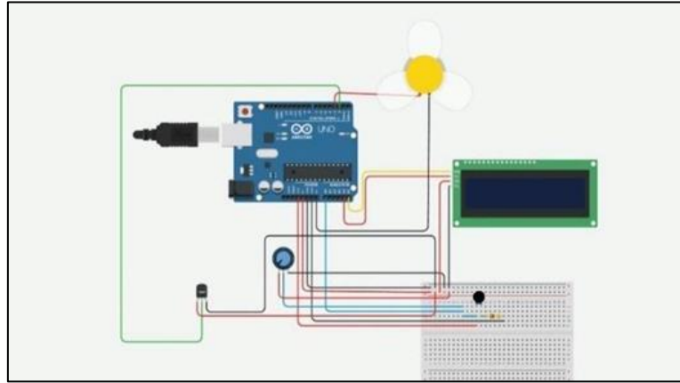
Figure 13. Simulation diagram
