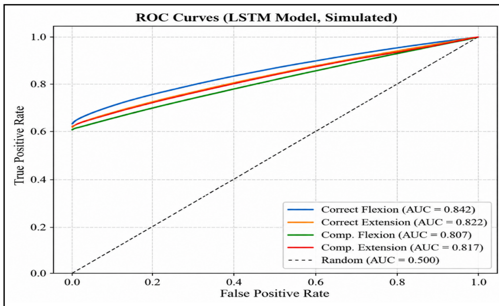
Figure 4. ROC curves of the proposed LSTM model for four-class Movement Classification
