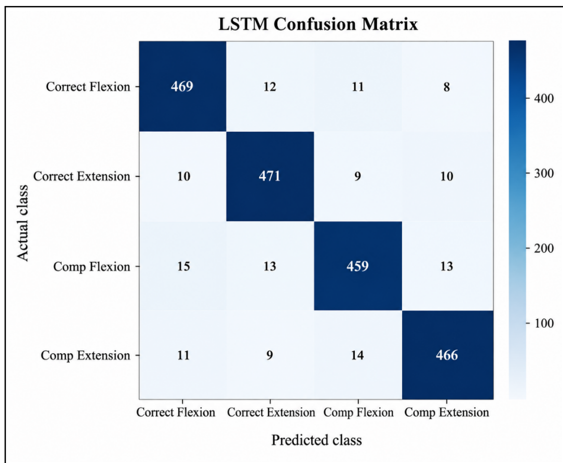
Figure 3. Confusion matrix of the LSTM-based movement classification
