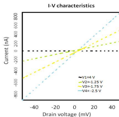
Figure 4. Performance of TMDC-based Bio-FET
