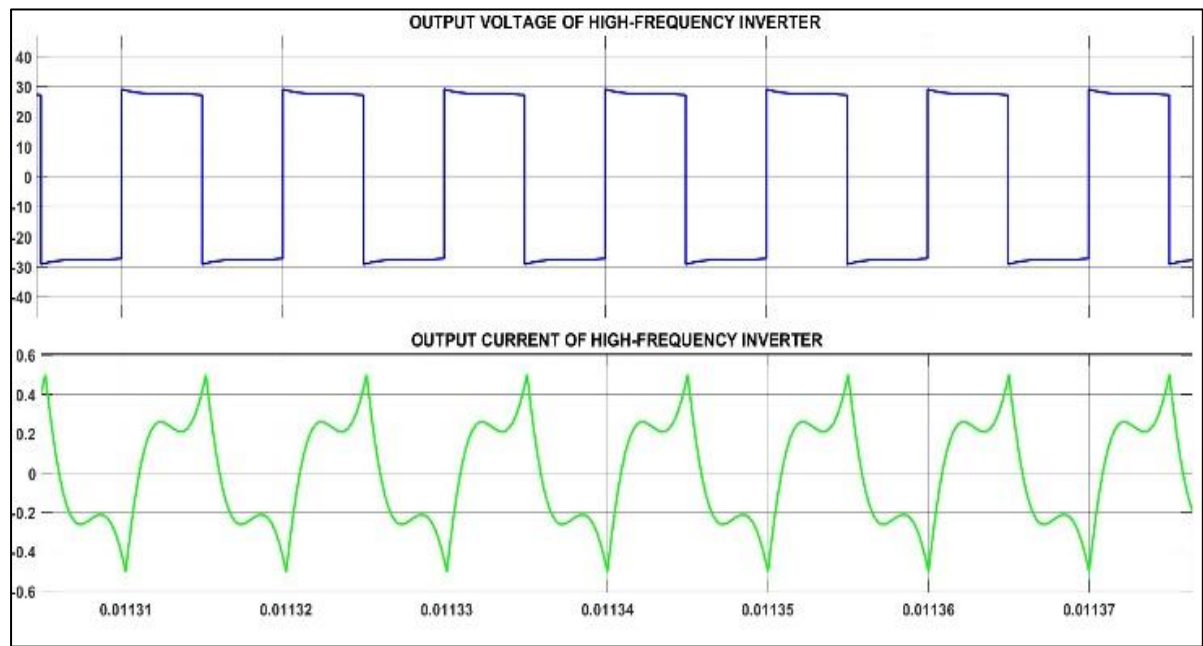
Figure 7. Transmitter Output
