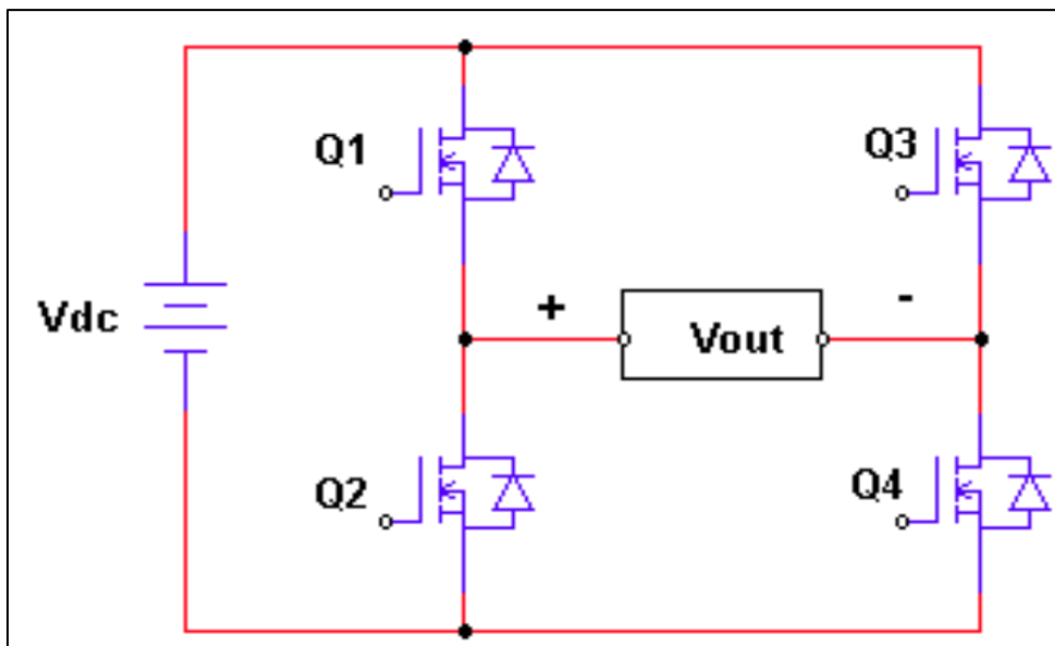
Figure 4. H-bridge Inverter[13]
