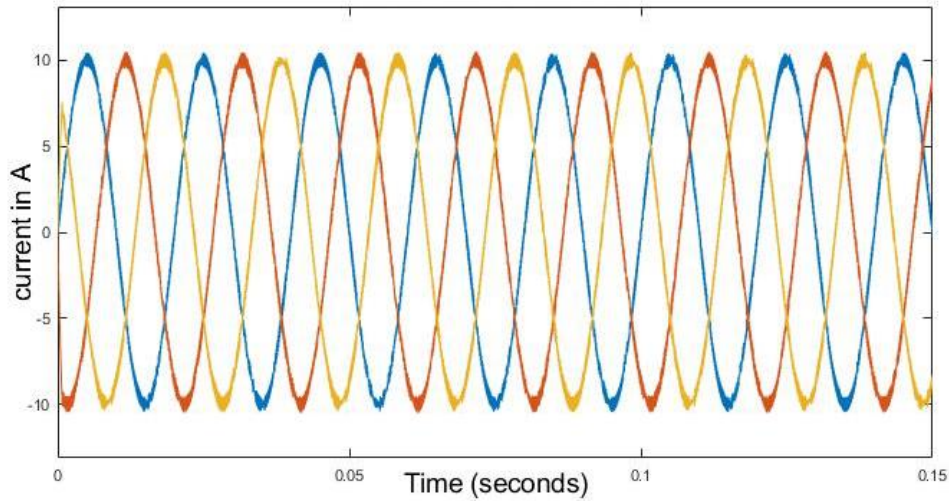
Figure 11. Line current at T_s=25\text{e-}6\text{ S}
