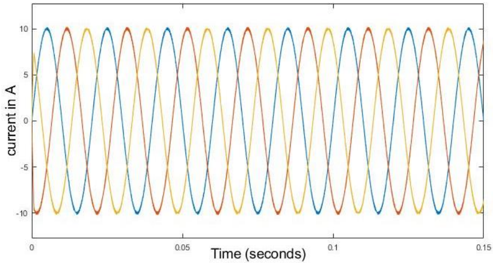
Figure 9. Line current at T_s=10\text{e-}6 S
