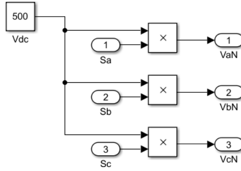
Figure 6. Inverter simlink model
