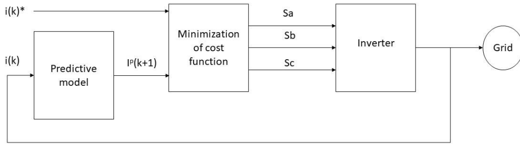
Figure 4. Block diagram
