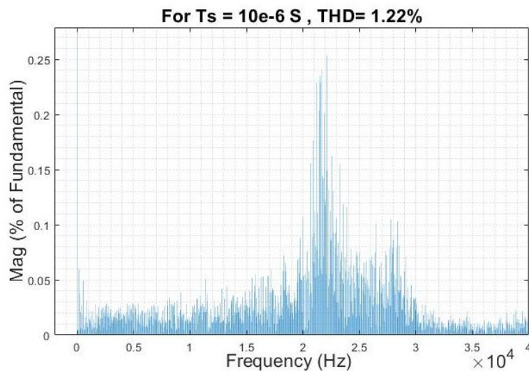
Figure 10. Line current THD at T_s=10\text{e-}6 S
