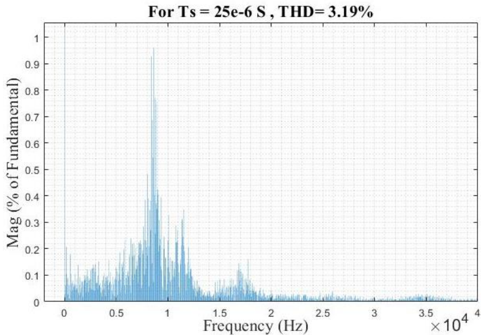
Figure 12. Line current THD at ( T_s=25\text{e-}6\text{ S} )
