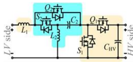
Figure 1. Non-isolated extendable bidirectional DC-DC converter
