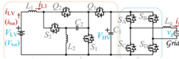
Figure 2. Existing Circuit
