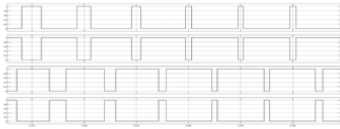
Figure 15. Output of Switching pulse of Inverter in boost mode
