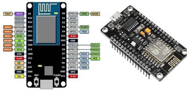
Figure 2. NodeMCU
