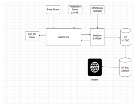
Figure 9. Block Diagram
