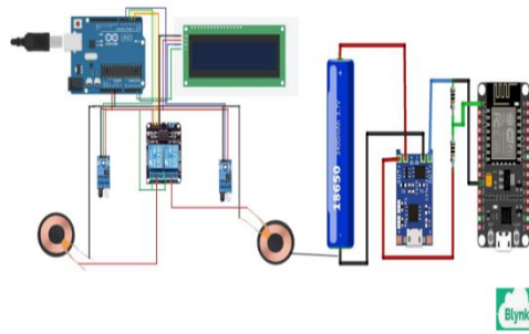
Figure 4. Circuit Diagram
