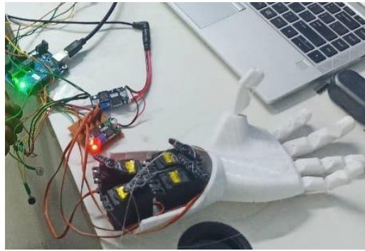
Figure 5. Prosthetic Hand
