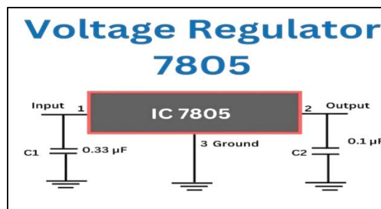
Figure 3. Voltage Regulator 7805
