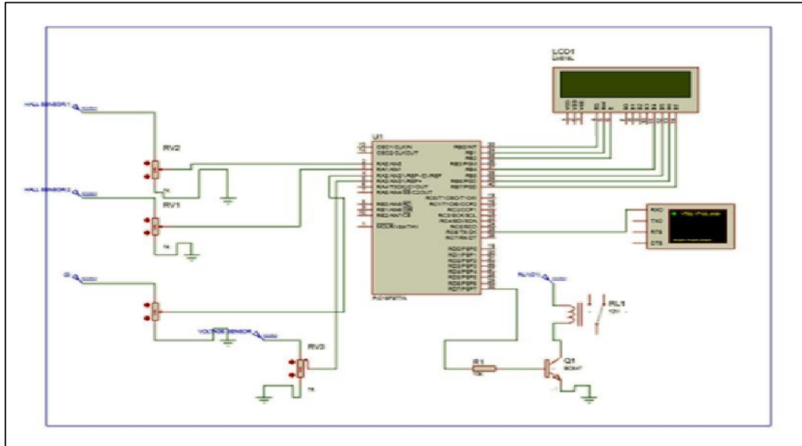
Figure 11. Circuit Diagram
