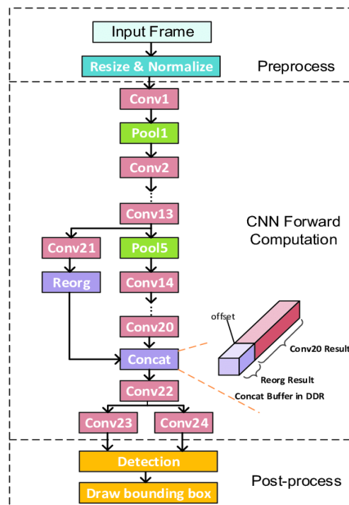
Figure 3.5. YOLO Functional Chart
