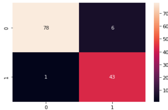
Figure 7. Confusion Matrix of Inception Model
