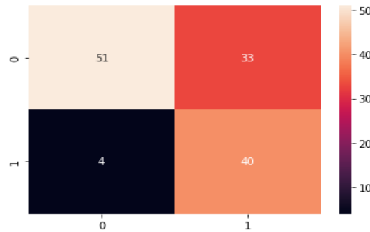
Figure 9. Confusion Matrix of the Resnet50 Model
