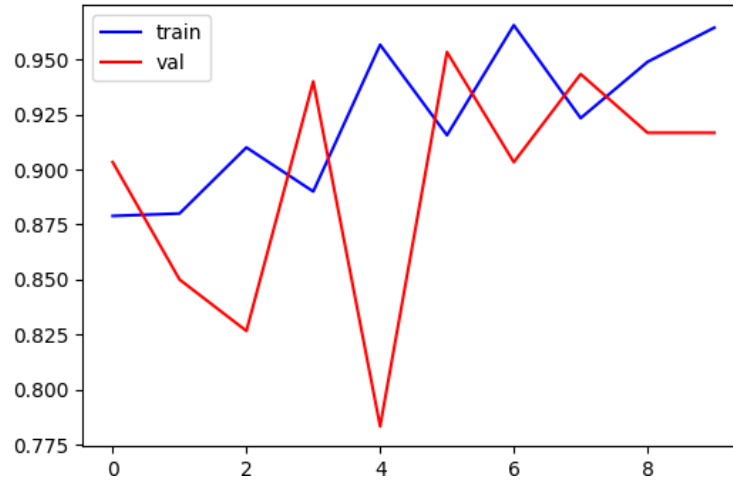
Figure 5. Accuracy Curve and Loss Curve
