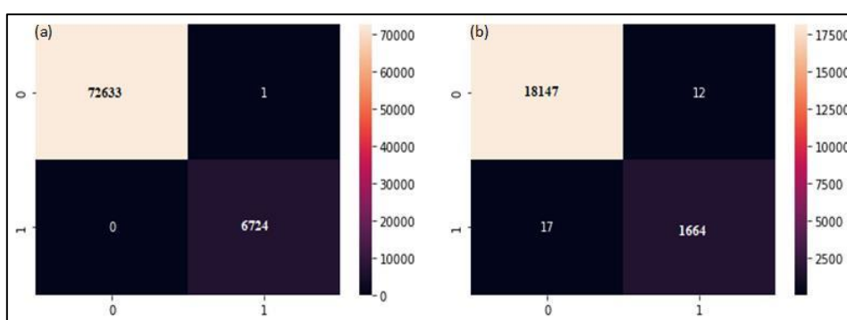
Figure 4: Shows a Confusion Matrix of Unbalanced Dataset using CNN+LSTM Method where (a) Represents Training Matrix while (b) Testing Matrix
