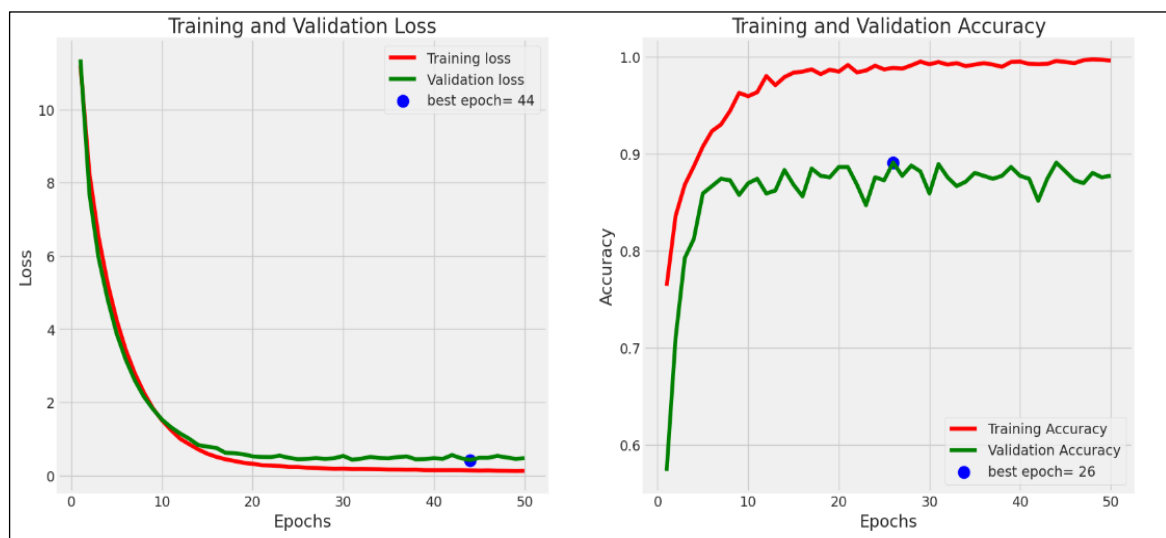
Figure 6. Loss and Accuracy Curves for Model 1
