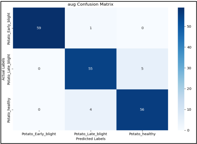
Figure 14. Confusion Matrix for Augmented Data
