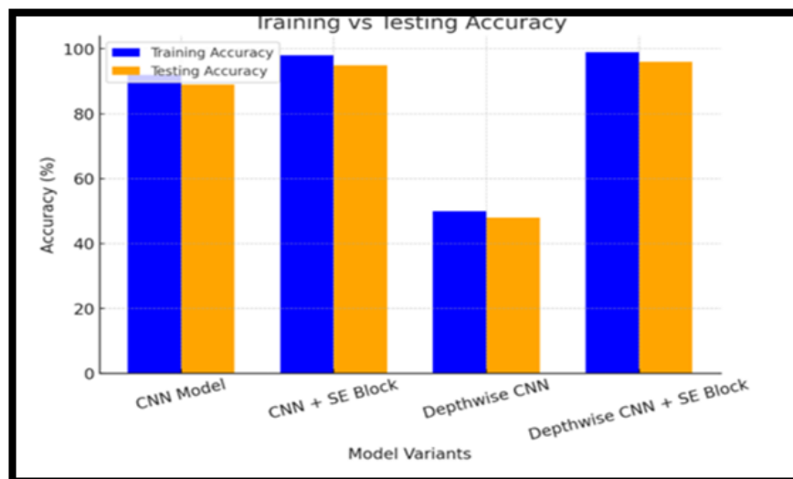
Figure 8. Accuracy Comparison of Different CNN Model Variants
