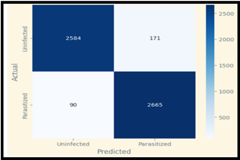
Figure 11. Confusion Matrix of XMal-CNN for Malaria Detection
