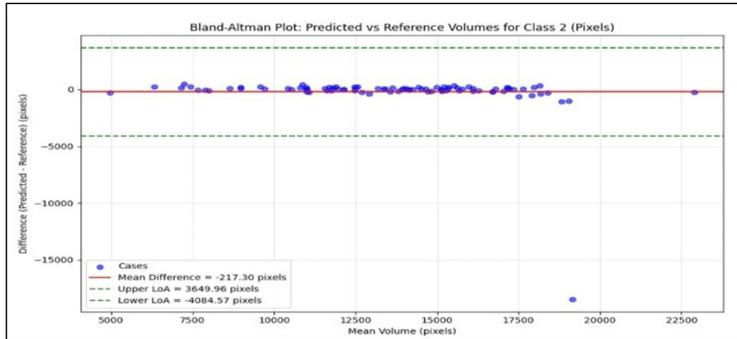
Figure 14. Bland-Altman for Class 2 (Left Lung), Shows the Difference (Predicted – Reference: Y-axis, -15,000 to 0) Versus the Mean (Mean Volume: X-axis, 5,000 to 22,500 Pixels)
