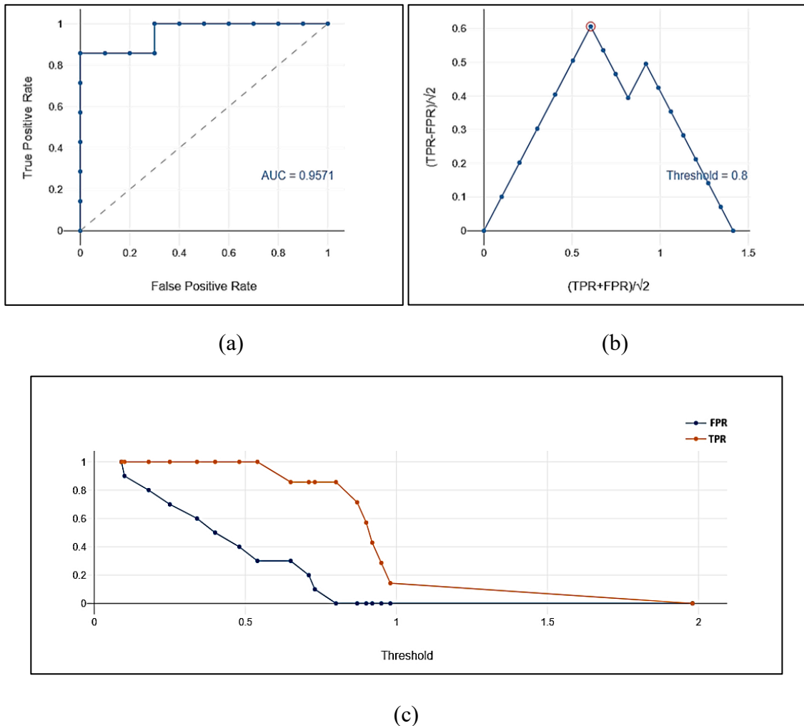
Figure 4. (a) Standard ROC Curve and AUC for Model Performance, (b) Rotated ROC Curve for Optimal Threshold Visualization, (c) FPR and TPR as a Function of Classification Threshold
