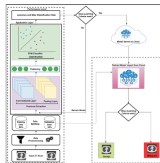
Figure 3. Block Diagram of the LungNet-SVM model [4].
