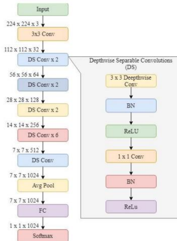
Figure 1. MobileNet Architecture [12]
