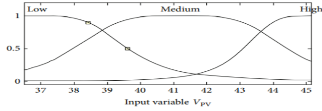
Figure 5. Membership function of the input variable ( V_{pv} )
