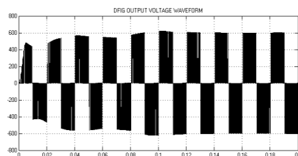
Figure 9. Output voltage for DFIG
