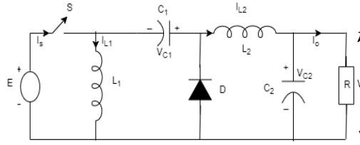
Figure 3. LUO Converter Circuit diagram
