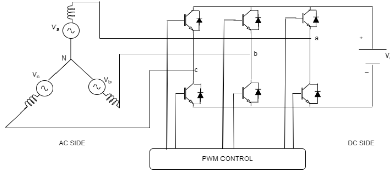
Figure 8. Three Phase PWM Rectifier
