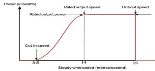
Figure 2. Typical wind turbine power output
