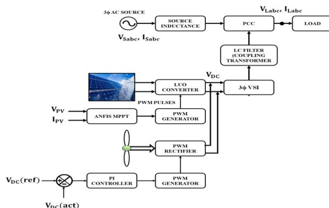
Figure 1. System under investigation
