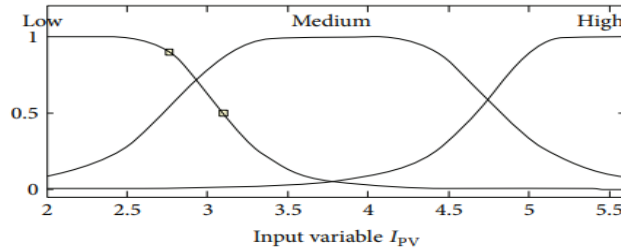
Figure 6. Membership function of the input variable ( I_{pv} )
