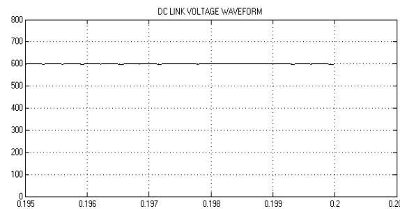
Figure 12. DC link voltage waveform
