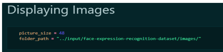
Figure 10. Code Implementation 2
