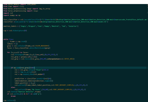
Figure 13. Code Implementation 5
