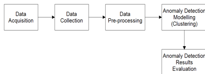
Figure 4. Data Analytics
