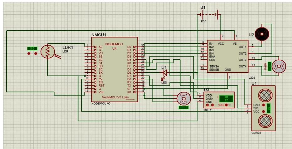
Figure 7. Circuit Diagram
