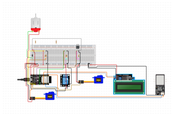
Figure 8. Circuit Diagram
