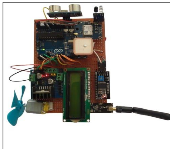
Figure 7. Prototype Model
