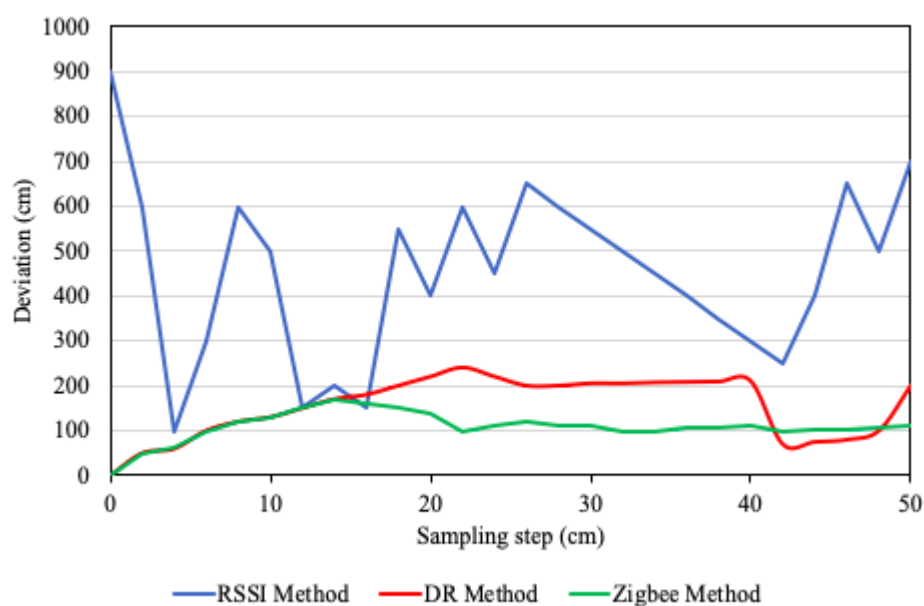
Figure 2. Comparison of localization error implementing RSSI, DR and Zigbee method
