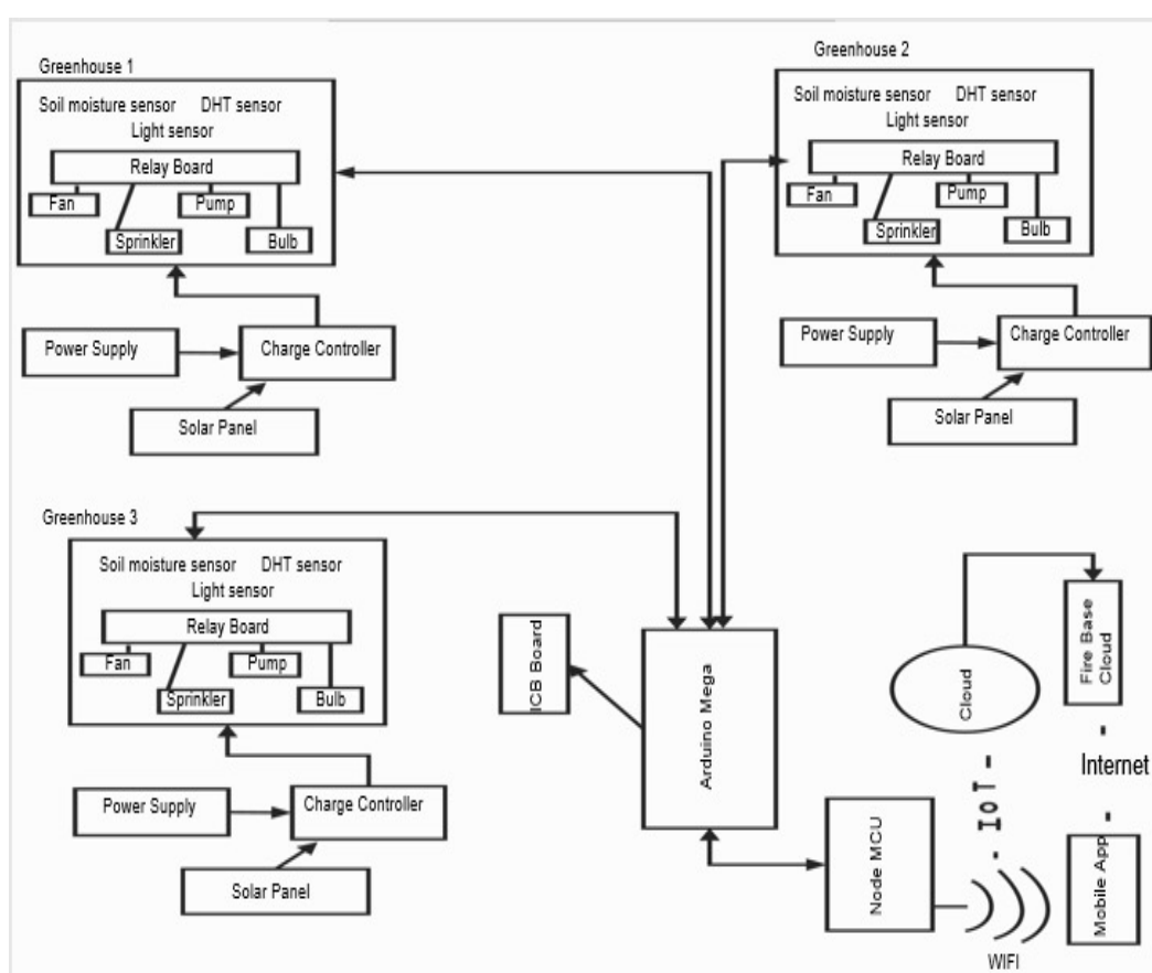
Figure 2. Block Diagram of the Model
