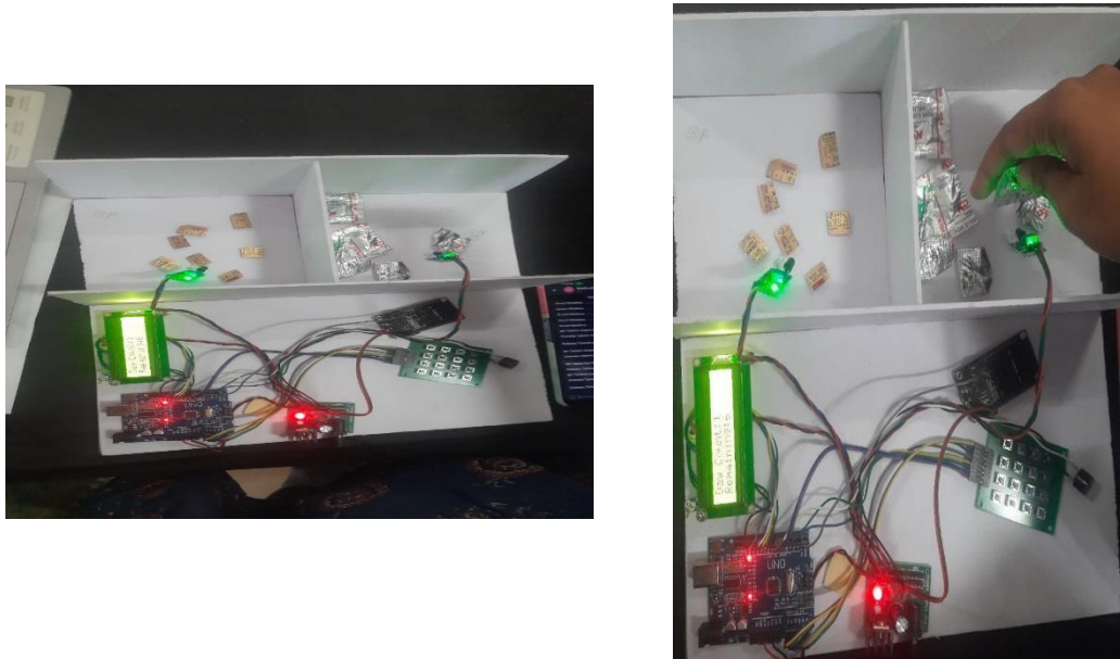
Figure 3. Hardware Prototype
