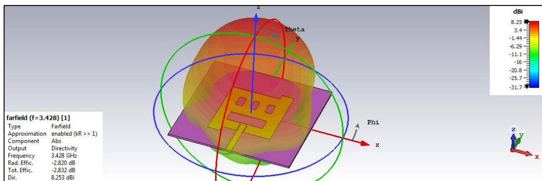
Figure 8. Directivity of Simulated Antenna at 3.42 GHz
