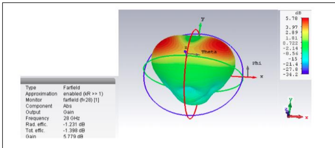
Figure 4. Radiation Pattern
